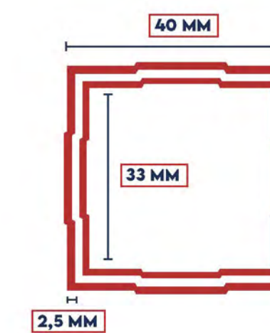
POTEAU DE COIN
